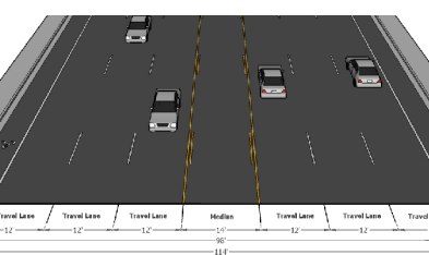
114' Principal Arterial
