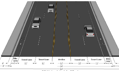
80' Major Arterial - Bike Lane (Travel Lane width 12', Buffer and/or 5' to 10'-12' on 15'-18' columns)
