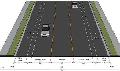
80' Major Collector - Buffered Bike Lane
