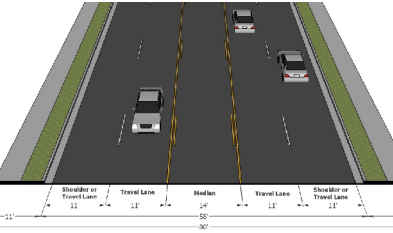
80' Major Arterial
