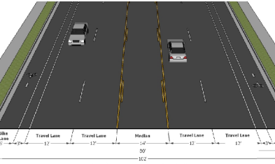
102' Major Arterial - Buffered Bike Lane
