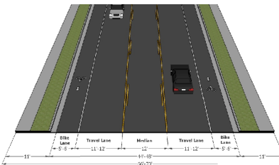
66'-70' Major Collector - Bike Lane (Asphalt width 48' unless noted)
