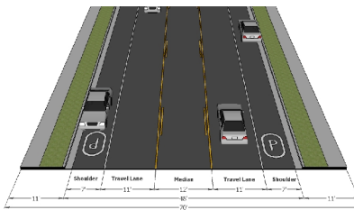
70' Major Collector
