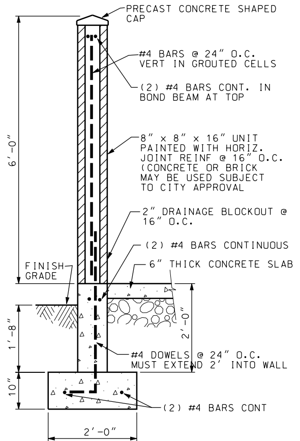
TRASH ENCLOSURE WALL DETAIL
